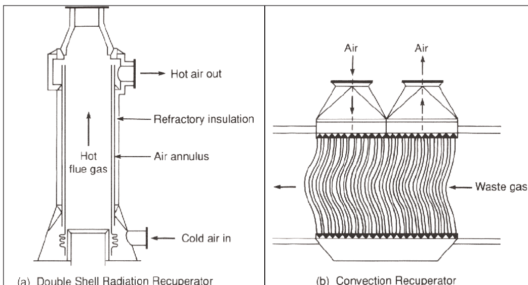
Figure 4.22 Metallic Recuperators
