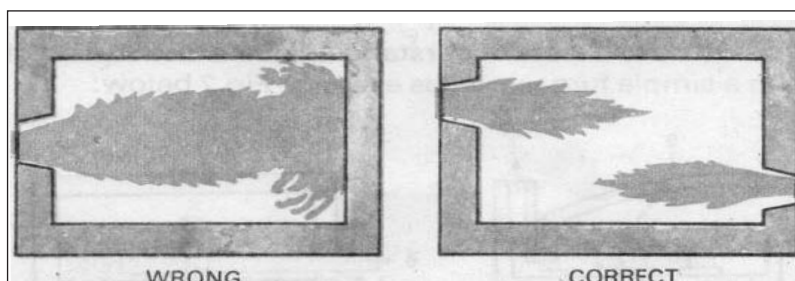
Figure 4.17 Heat Distribution in Furnace
