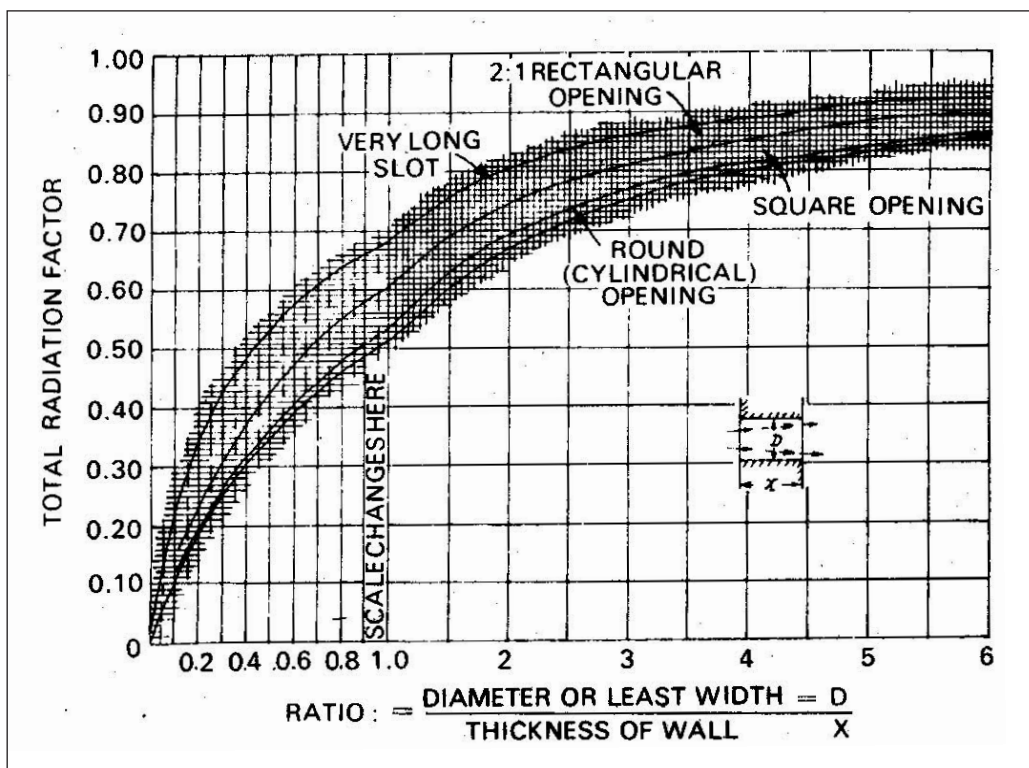
Figure 4.13 Factor for Determining the Equivalent of Heat Release from Openings to the Quality of Heat Release from Perfect Black Body
