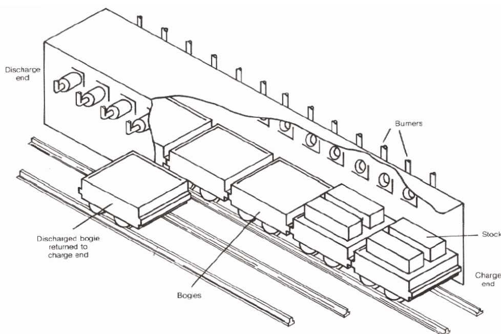
Figure 4.7 Continuous circulating bogie type furnace
