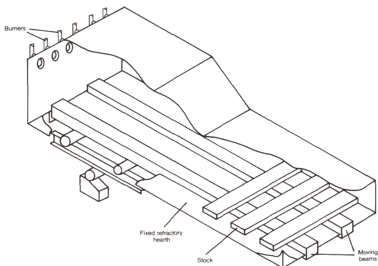
Figure 4.5 Walking Hearth Type Furnace
