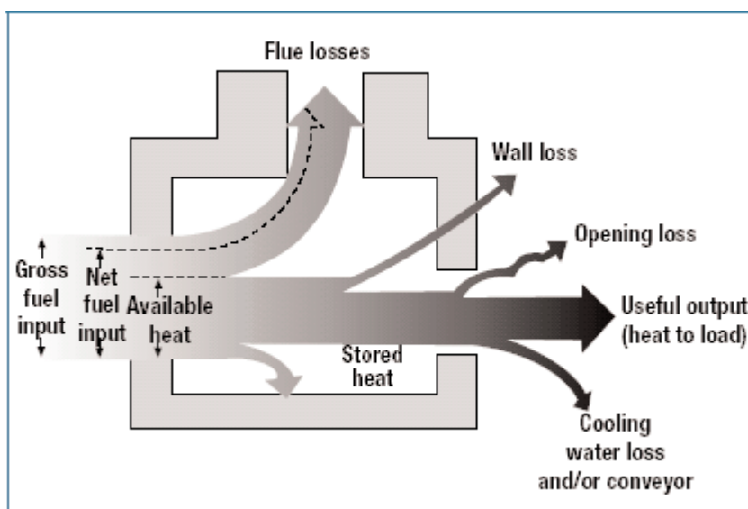
Figure 4.9 Heat Losses in Industrial Heating Furnaces
