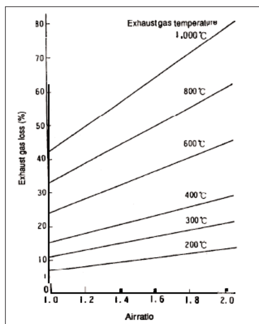
Figure 4.15 Relation Between Air Ratio and Exhaust Gas Loss
