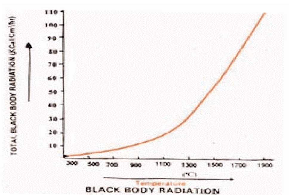
Figure 4.14 Graph for Determining Black Body Radiation at a Particular Temperature
