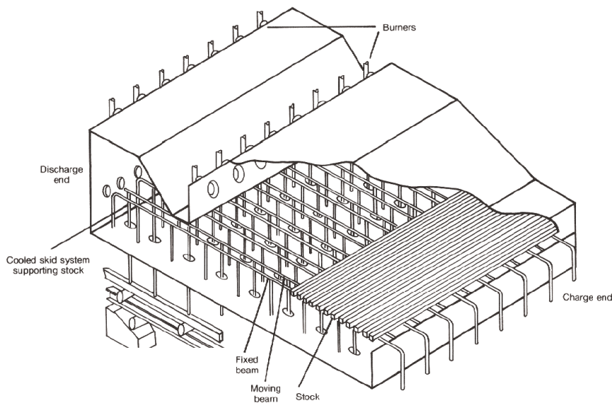
Figure 4.8 Walking Beam Type Furnace
