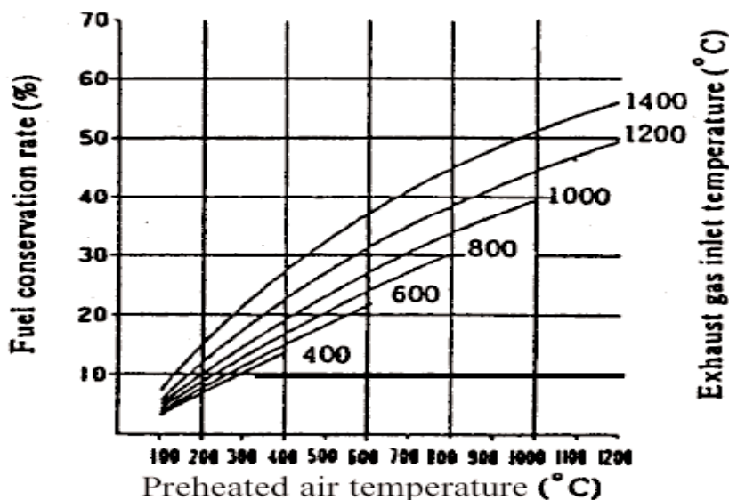
Figure 4.25 Fuel Conservation Rate when Natural Gas is Used
