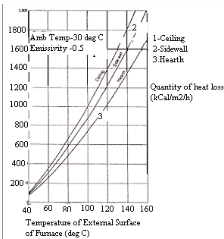
Figure 4.26 Quantity of Heat Release at Various Temperatures
