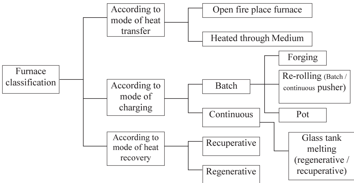
Figure 4.1: Furnace Classification
