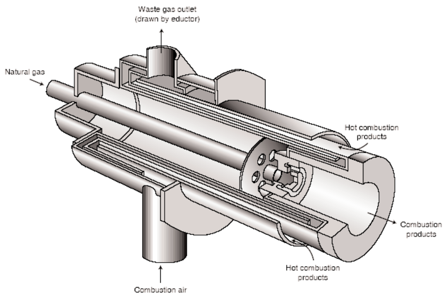
Figure 4.23 Self-Recuperative Burners
