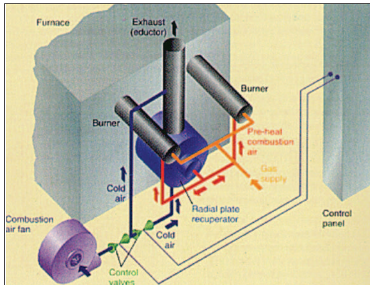
Figure 4.21 Preheating the Air for Combustion by a Recuperator
