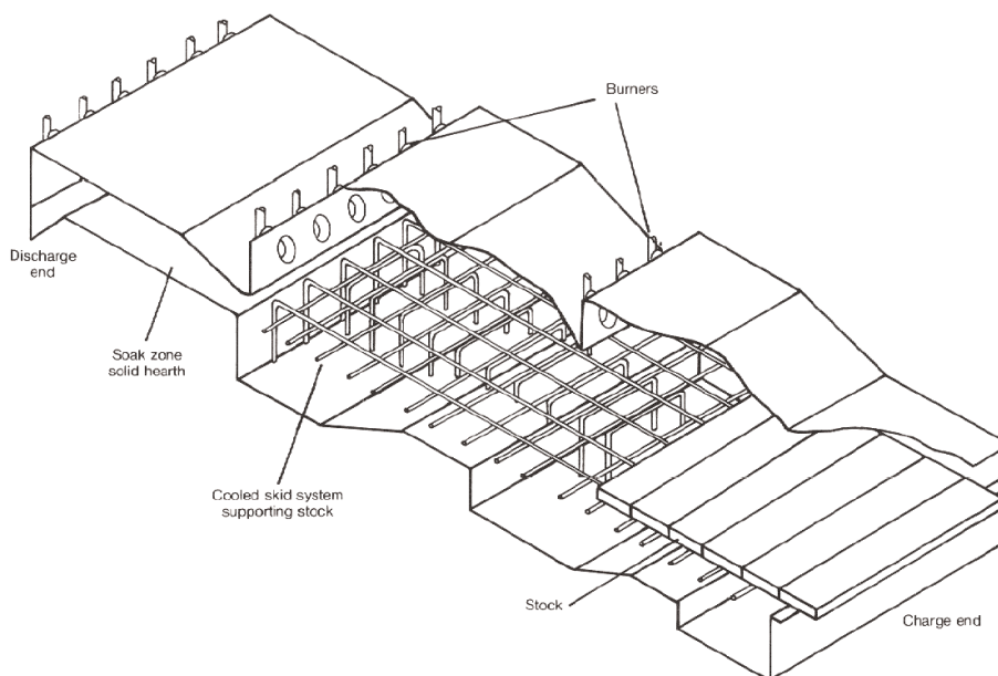
Figure 4.4 Pusher Type Furnaces
