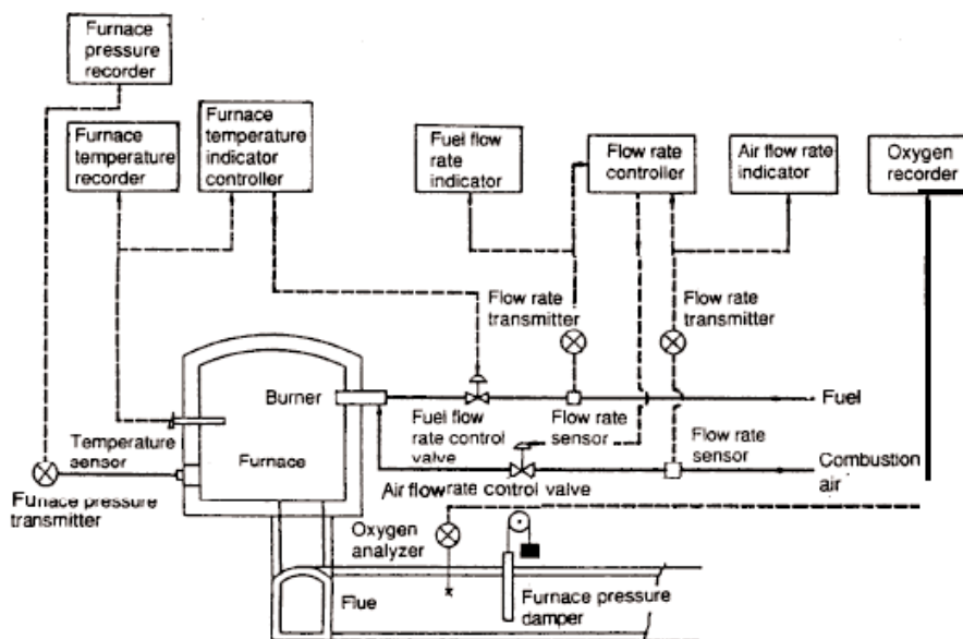
Figure 4.16 Air/Fuel Ratio Control System with Flow Rate Controller
