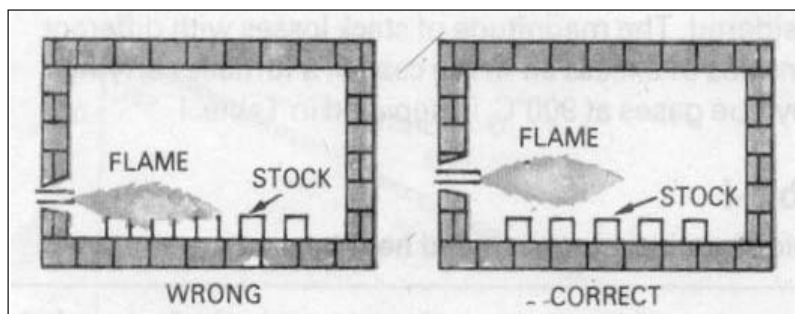
Figure 4.18 Alignment of Burners in Furnace
