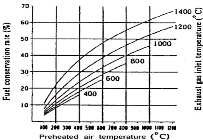
Figure 4.24 Fuel Conservation Rate when Oil is Used
