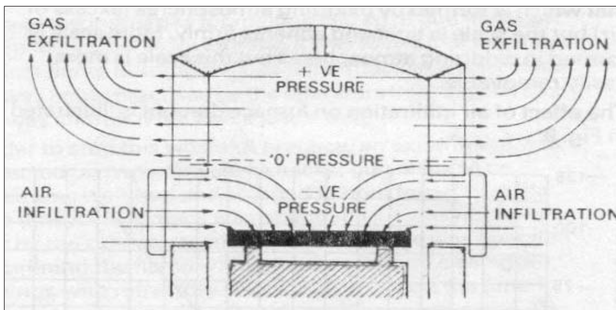
Figure 4.19 Effect of Pressure on the Location of Zero Level and Infiltration of Air
