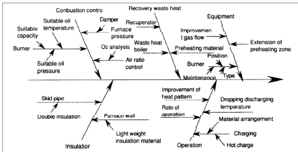
Figure 4.27 Characteristic Diagram of Energy Conservation for Reheating Furnace
